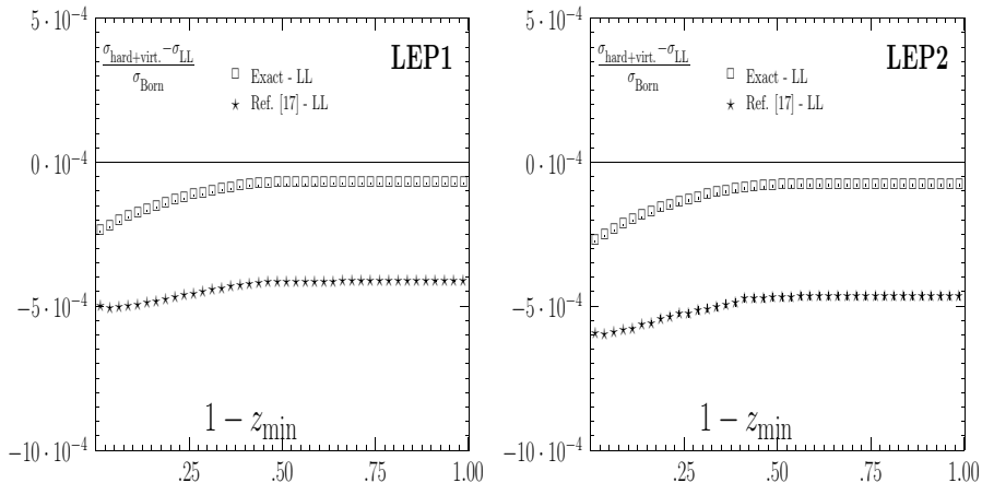
Fig. 1. Monte Carlo results ( 10^6 events) for the \mathcal{O}(\alpha^2) cross section for single photon emission from the electron line. Differences between three matrix elements are shown for the SICAL Wide-Narrow trigger, divided by the Narrow-Narrow Born cross section, with z_{\min} defined as in Fig. 2 of Ref. [18]. The two graphs display results for LEP1 and LEP2 parameters, respectively.
