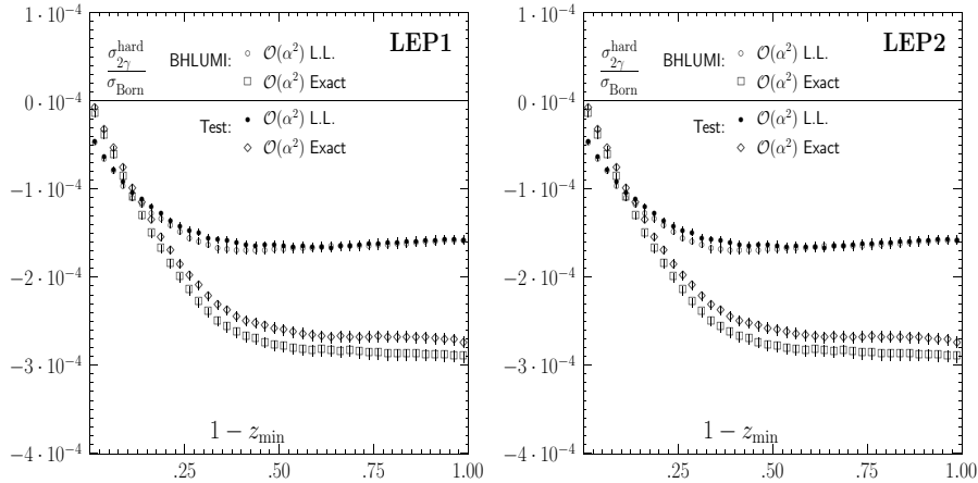
Fig. 2. Monte Carlo results ( 10^6 events) for the \mathcal{O}(\alpha^2) cross section for photon emission from the electron line. Exact and leading log hard photon cross sections are shown for the SICAL Wide-Narrow trigger, divided by the Narrow-Narrow Born cross section, with z_{\min} defined as in Fig. 2 of Ref. [18]. The two graphs display results for LEP1 and LEP2 parameters, respectively.
