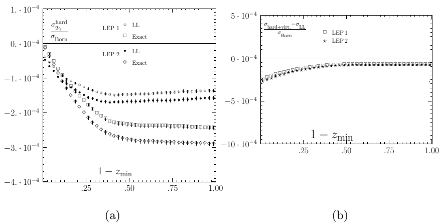
Figure 1. Monte Carlo results ( 10^6 events) for the O(\alpha^2) cross section for (a) two hard photon emission and (b) single hard plus virtual photon emission from the electron line for LEP1 and LEP2 parameters, where z_{\min} is a lower bound on the fraction of the beam energy carried away by the electron and positron. The cross sections are normalized by dividing by the Born cross section, and in (b), the leading log contribution is subtracted.
