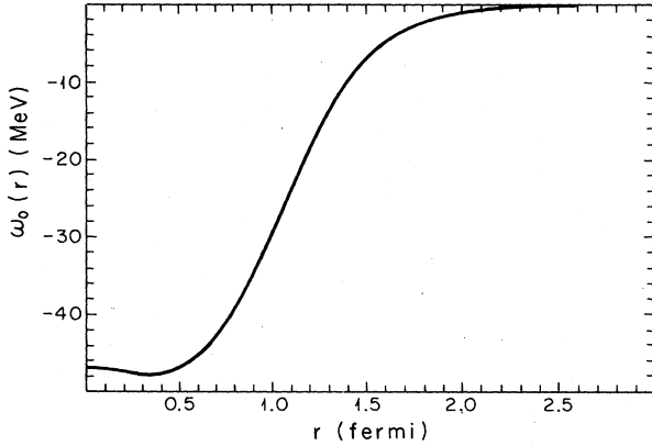
FIG. 2. The omega field \omega_0 for F_\pi = 124 MeV and \beta = 15.6 .
